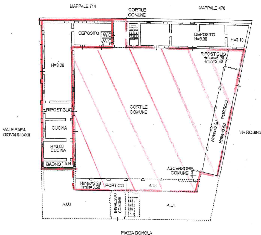
PIANO TERRA
